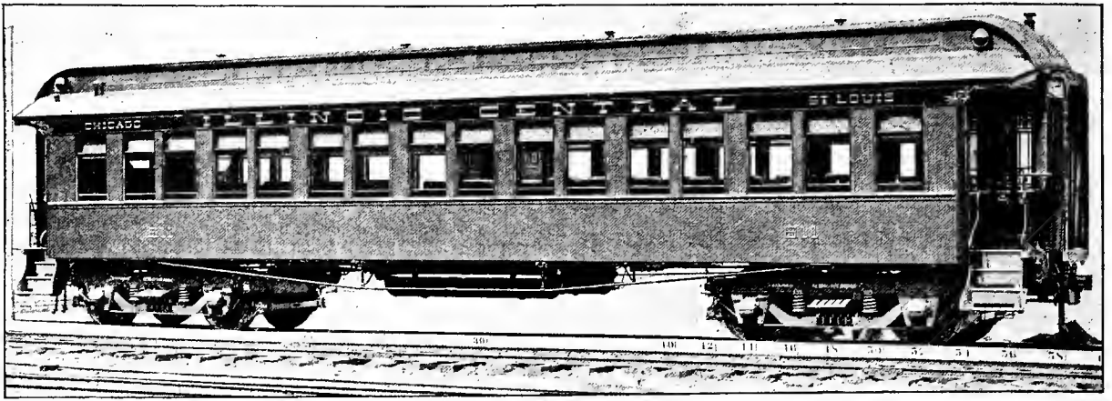
Fig. 89. COACH, FIRST-CLASS, WITH SMOKING COMPARTMENT. ILLINOIS CENTRAL RAILROAD. Length, 51 ft. 6 ins. Capacity, 56 persons. Weight, 60,900 lbs.
